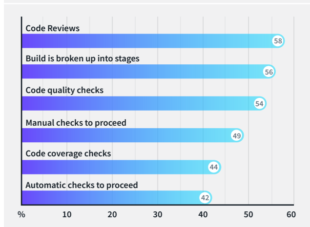
GRAPH 01. Top 6 Software Delivery Processes
